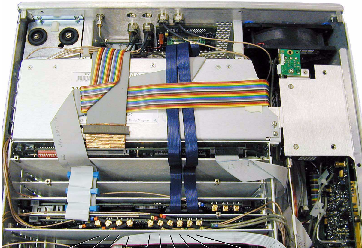
Figure 2-46 A35 3-20 GHz I/Q Modulator
