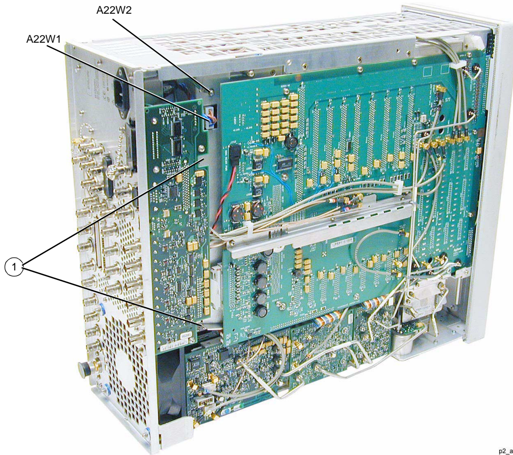
Figure 2-21 Rear Panel Removal (Option 1EM)
