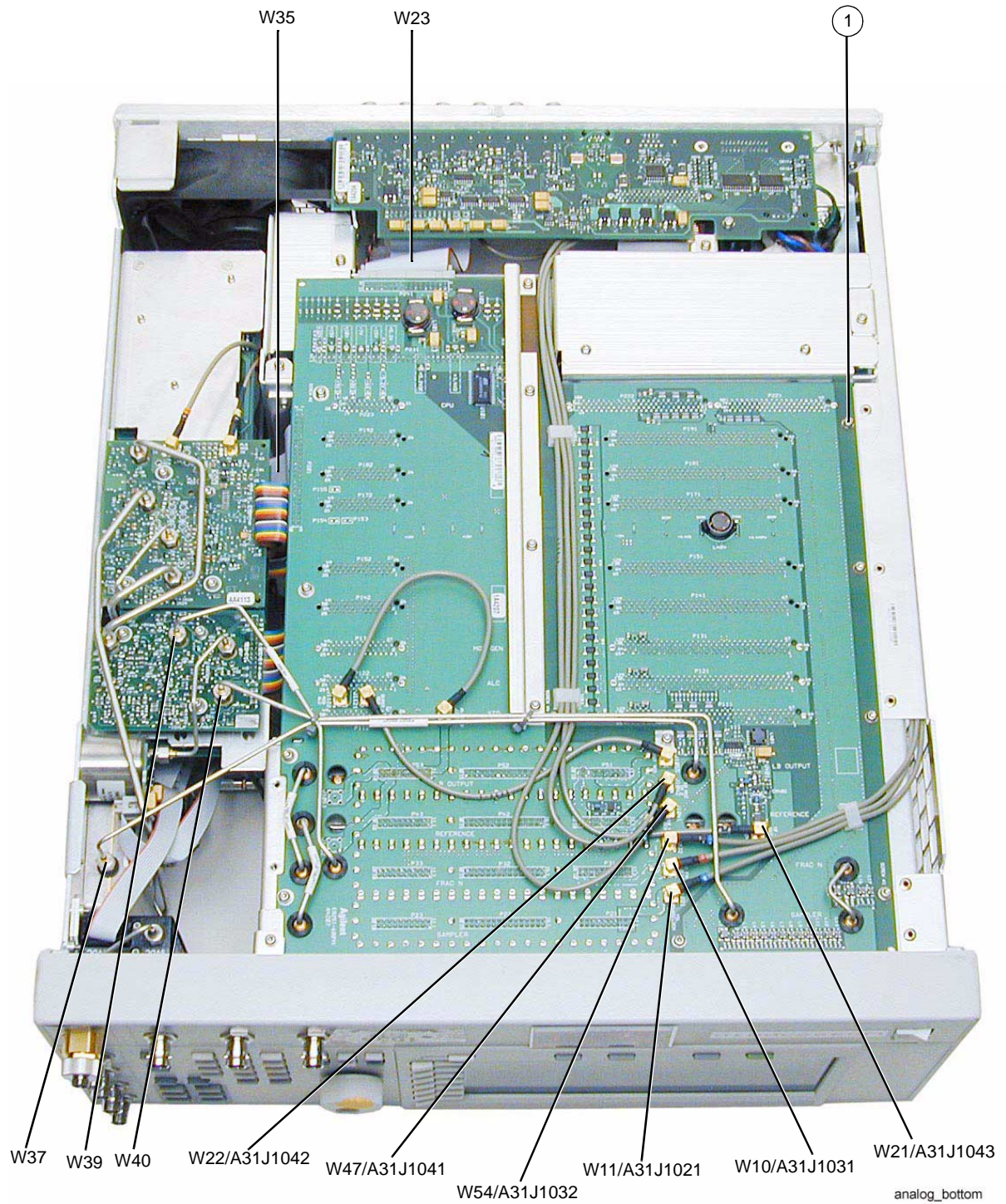
Figure 2-41 A31 Motherboard (E8247C/57C)
